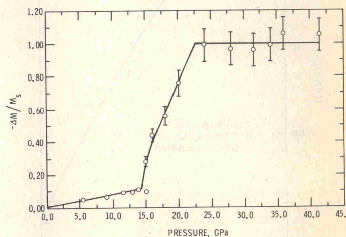
FIG. 22. The indicated relative change in magnetization, M_s , for various shock loading pressures for Fe-3.25 wt% Si shows a phase transition to a nonferromagnetic phase beginning at about 14 GPa. The data indicate that the transition is complete at 22.5 GPa. The apparent magnetization change below the transition is that expected from stress-induced magnetic anisotropy and the change in magnetization with pressure for the bcc phase. The figure illustrates how experiments conducted at closely spaced input pressure can provide independent data on details of ferromagnetic to nonferromagnetic transitions. From Graham (1968).
